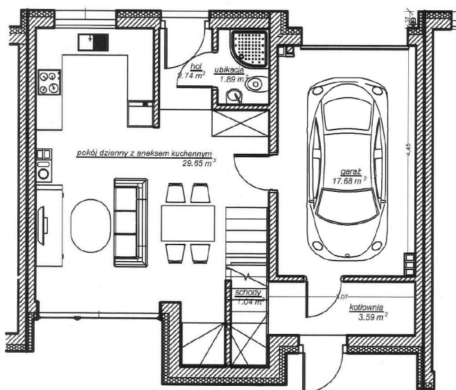
PARTER
